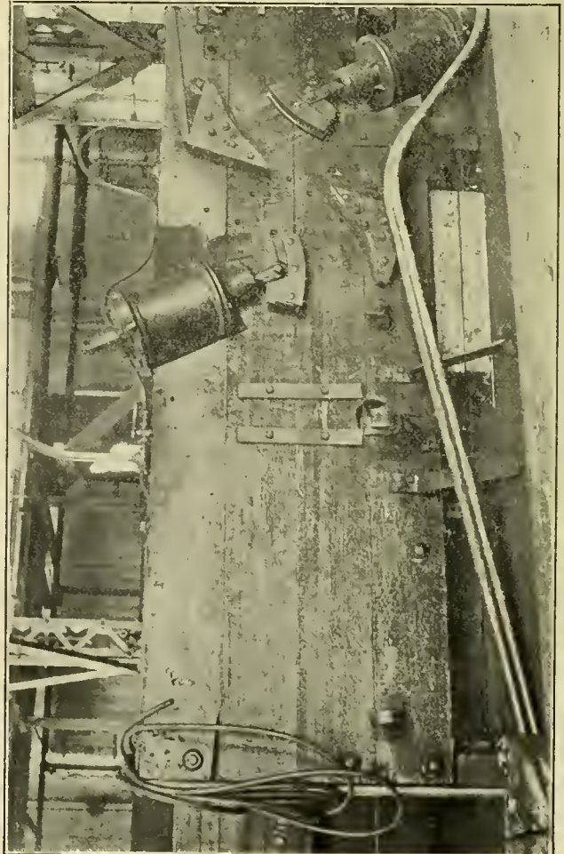
FIG. 69.—PNEUMATIC DEVICE FOR BENDING BRAKE LINES COMPLETE IN ONE OPERATION.
